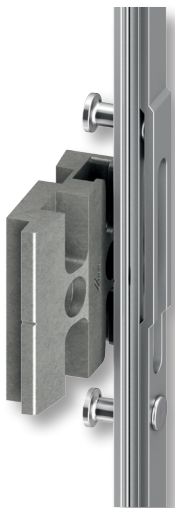
Mushrooms locate into both sides of striker plate
